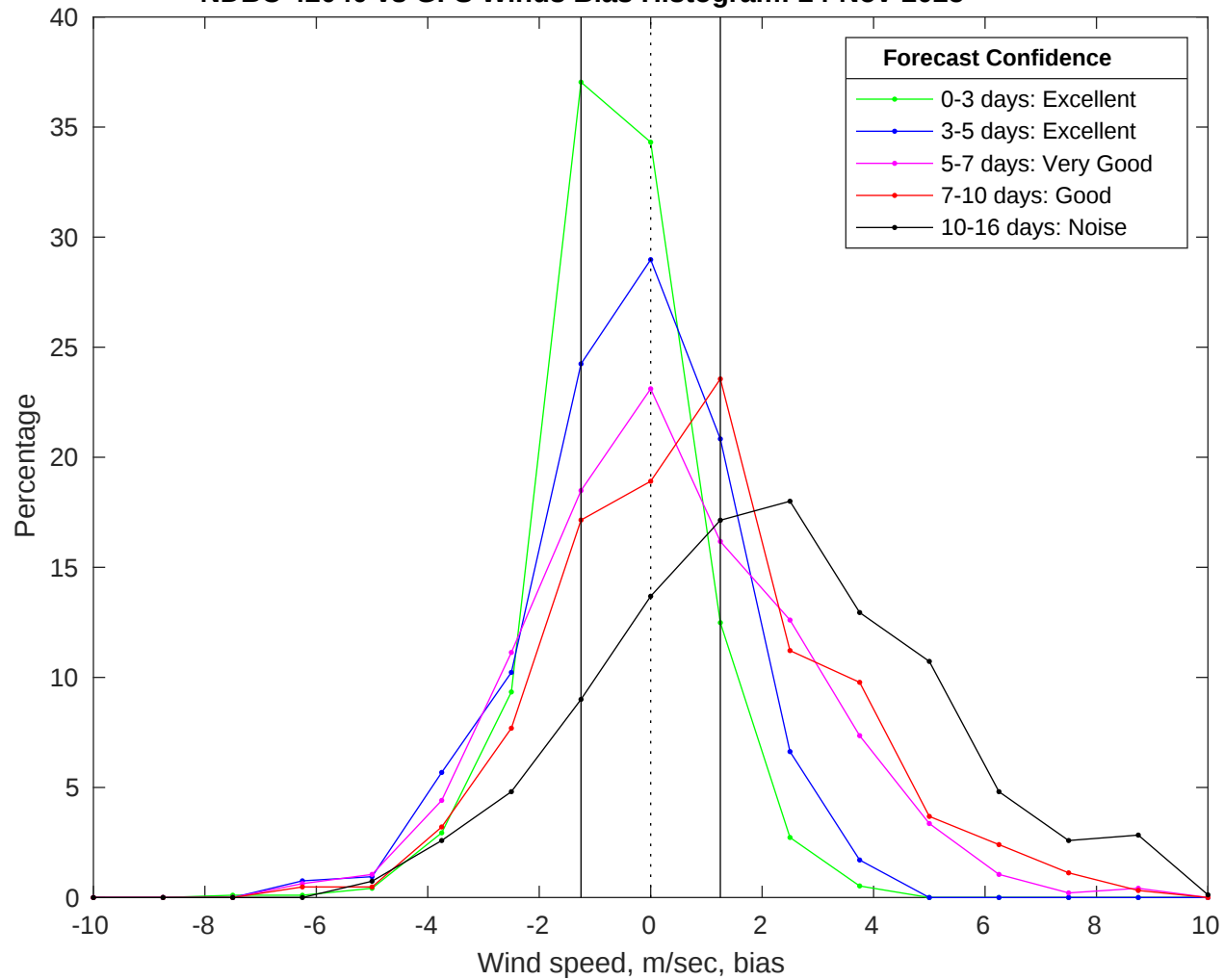
NDBC 42040 vs GFS Winds Bias Histogram: 24-Nov-2025
