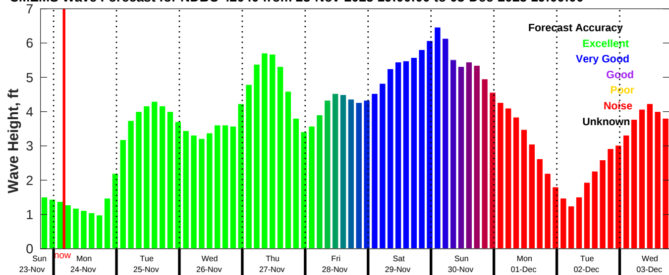
CMEMS Wave Forecast for NDBC 42040 from 23-Nov-2025 19:00:00 to 03-Dec-2025 19:00:00
