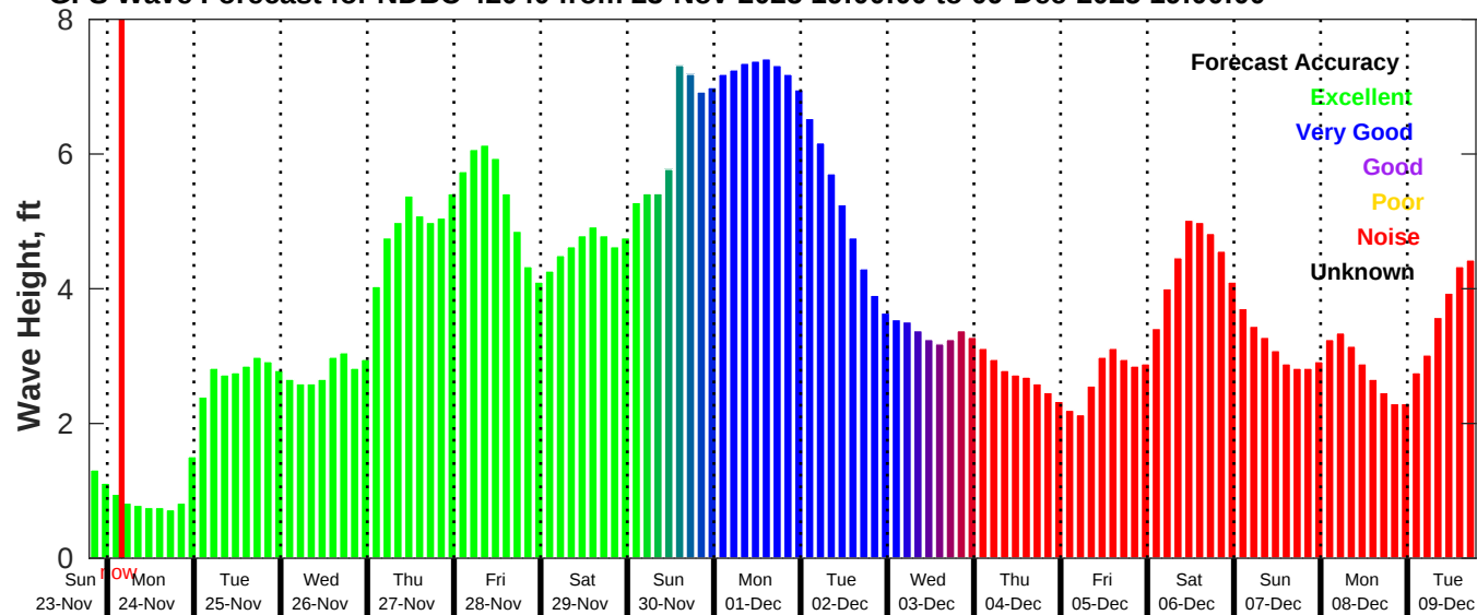
GFS Wave Forecast for NDBC 42040 from 23-Nov-2025 19:00:00 to 09-Dec-2025 19:00:00
