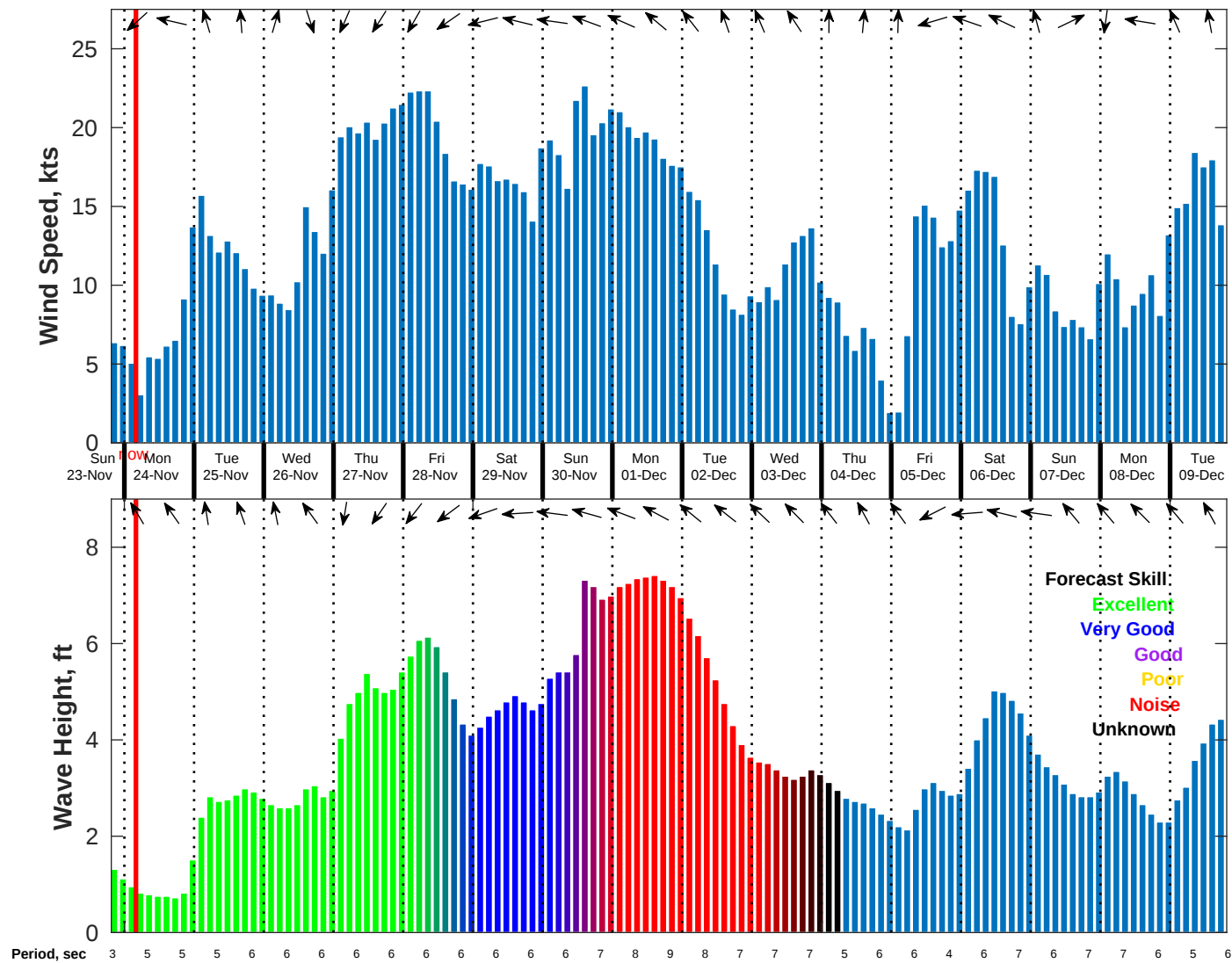
Wind & Wave Forecast for NDBC 42040 from 23-Nov-2025 19:00:00 to 09-Dec-2025 19:00:00
