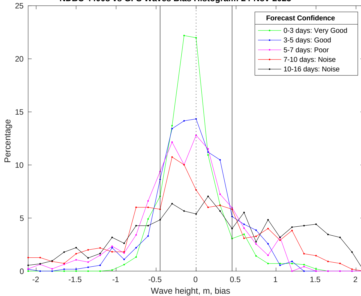
NDBC 44008 vs GFS Waves Bias Histogram: 24-Nov-2025
