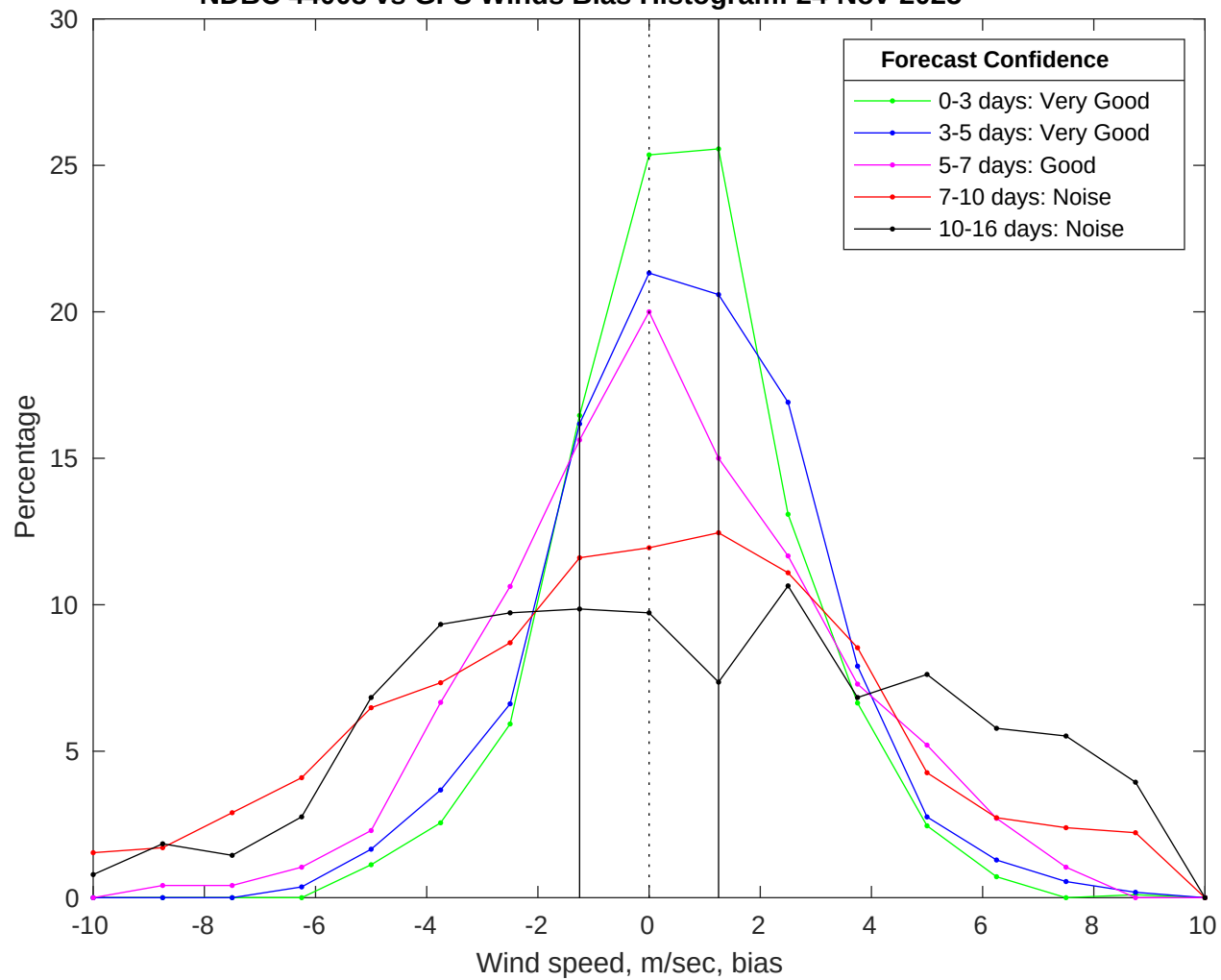
NDBC 44008 vs GFS Winds Bias Histogram: 24-Nov-2025
