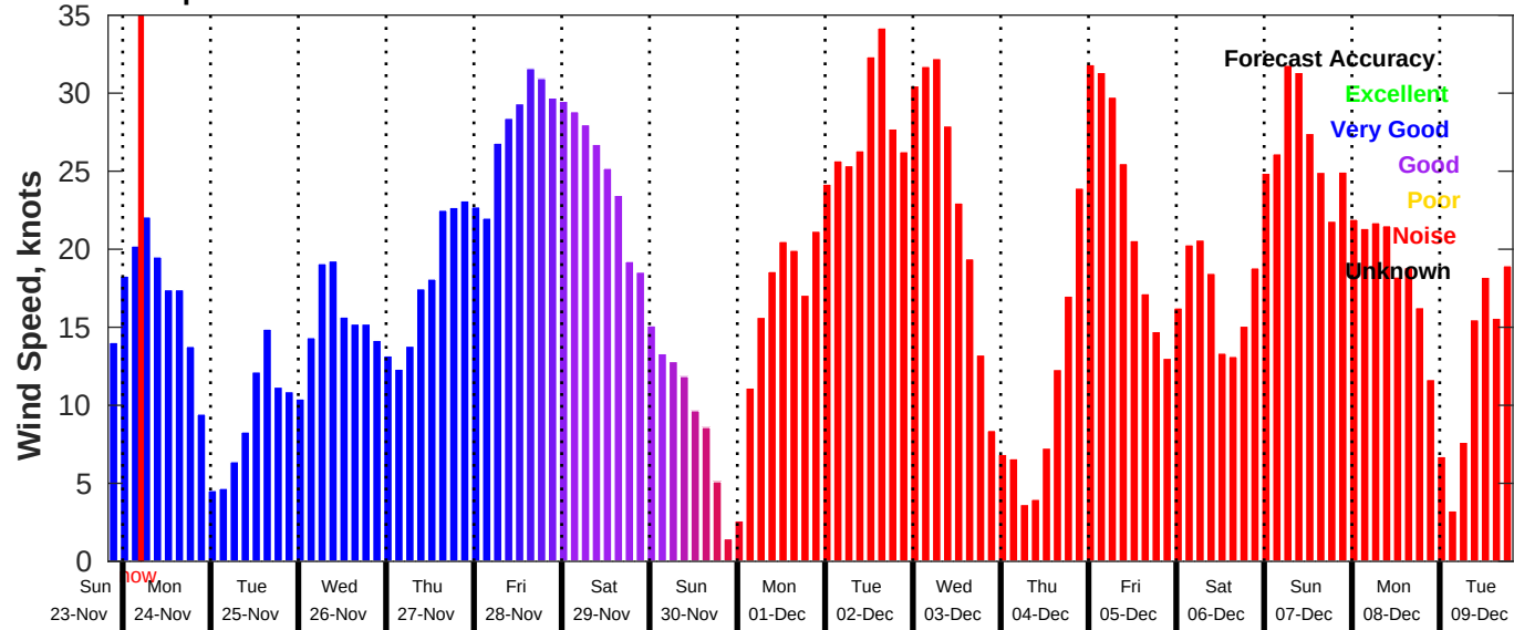
GFS Wind Speed Forecast for NDBC 44008 from 23-Nov-2025 20:00:00 to 09-Dec-2025 20:00:00
