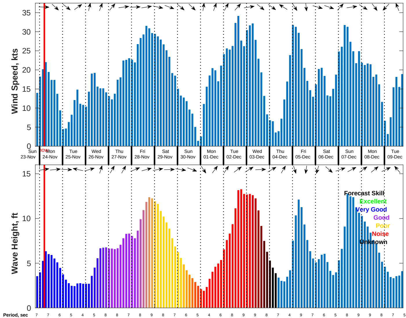
Wind & Wave Forecast for NDBC 44008 from 23-Nov-2025 20:00:00 to 09-Dec-2025 20:00:00
