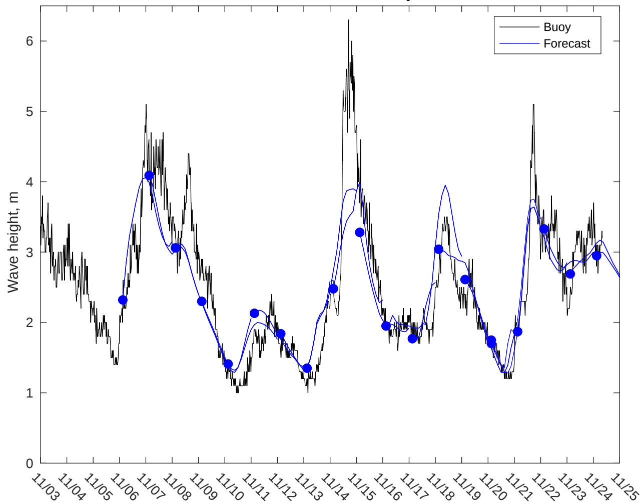
NDBC 46011 vs CMEMS Waves: 3 to 5 day forecast
