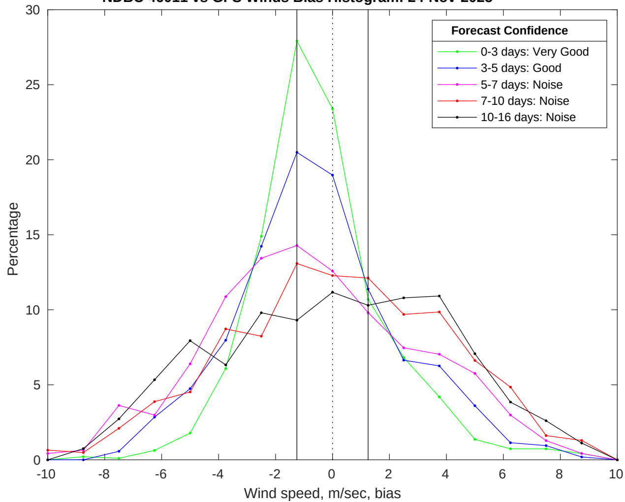
NDBC 46011 vs GFS Winds Bias Histogram: 24-Nov-2025
