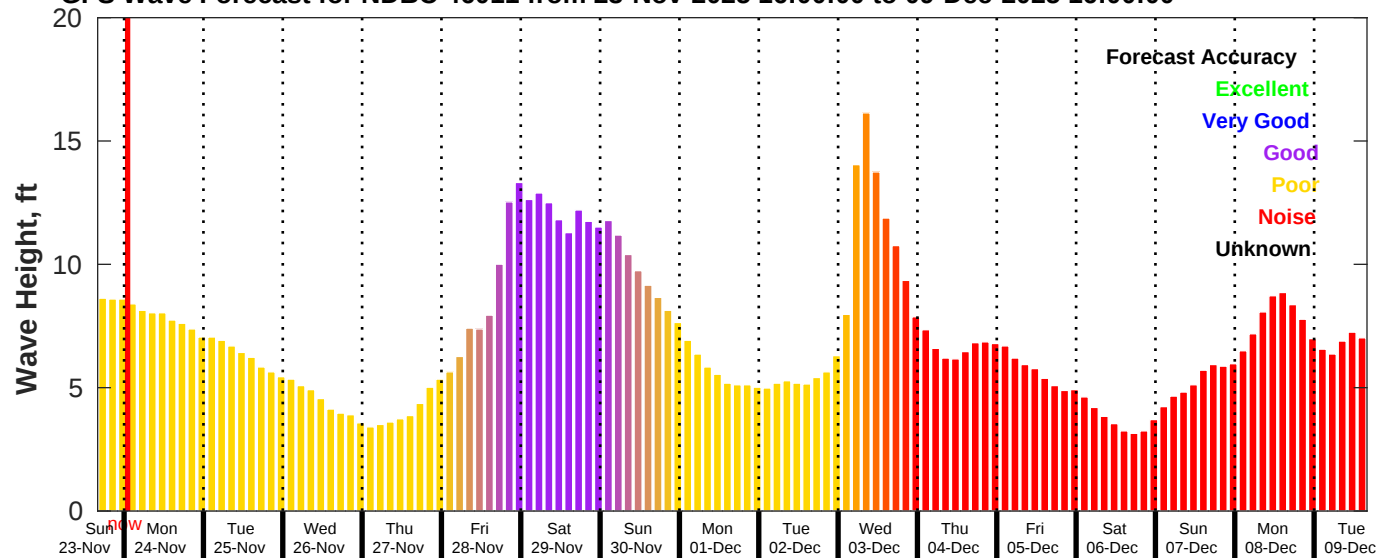
GFS Wave Forecast for NDBC 46011 from 23-Nov-2025 16:00:00 to 09-Dec-2025 16:00:00
