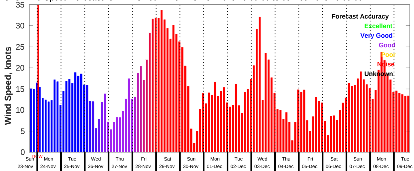
GFS Wind Speed Forecast for NDBC 46011 from 23-Nov-2025 16:00:00 to 09-Dec-2025 16:00:00
