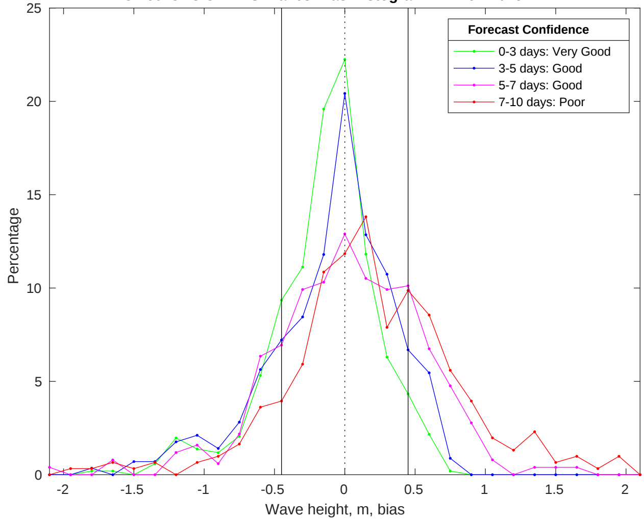
NDBC 46028 vs CMEMS Waves Bias Histogram: 24-Nov-2025
