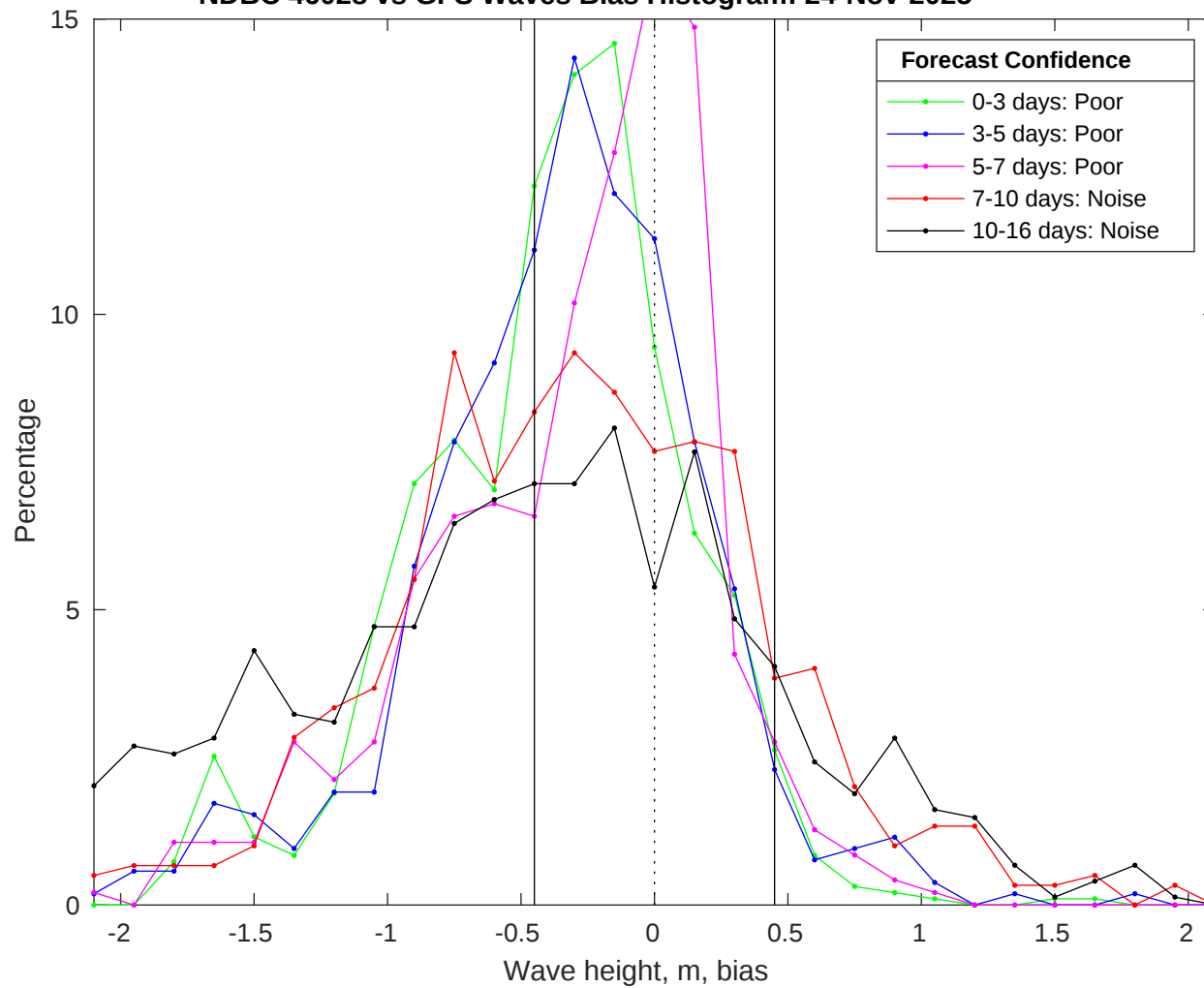
NDBC 46028 vs GFS Waves Bias Histogram: 24-Nov-2025
