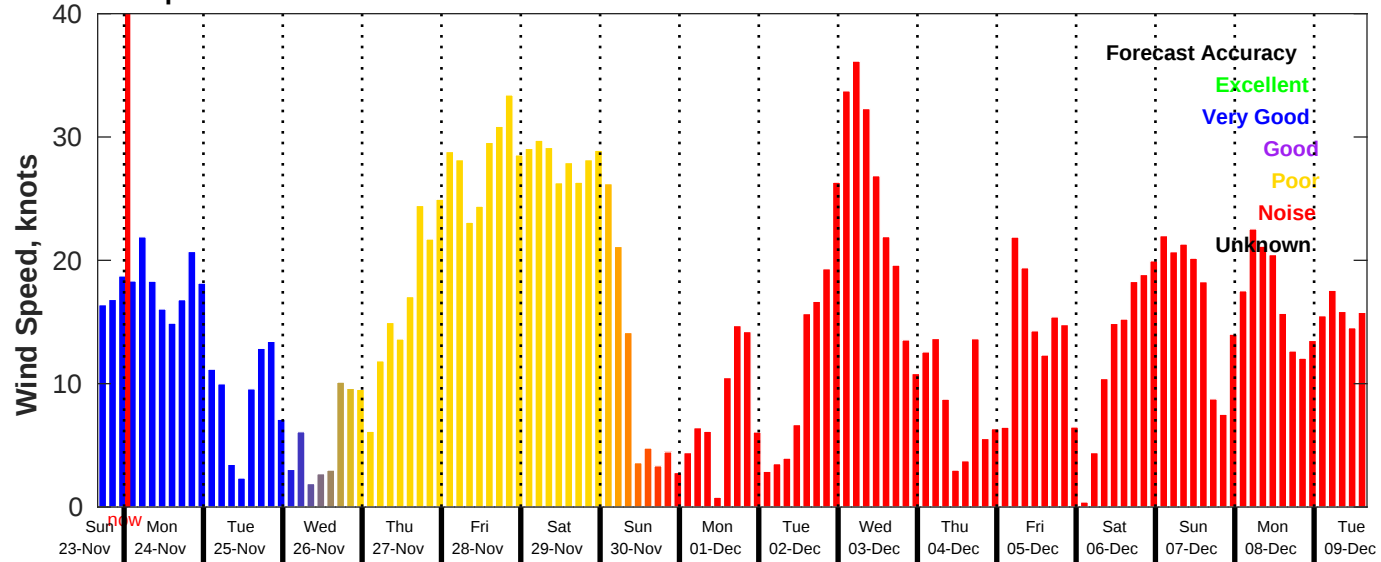
GFS Wind Speed Forecast for NDBC 46028 from 23-Nov-2025 16:00:00 to 09-Dec-2025 16:00:00
