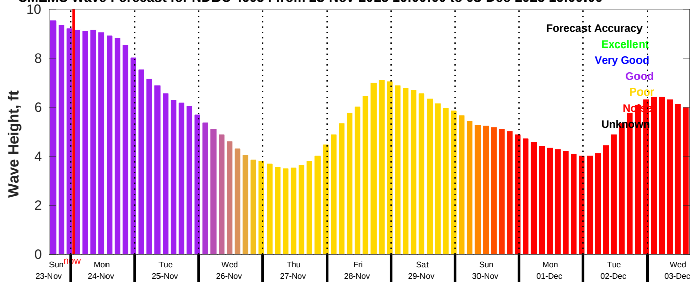
CMEMS Wave Forecast for NDBC 46054 from 23-Nov-2025 16:00:00 to 03-Dec-2025 16:00:00
