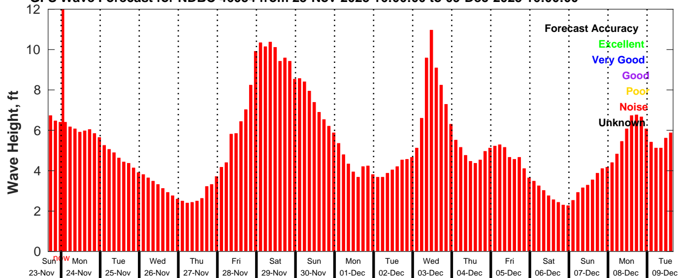
GFS Wave Forecast for NDBC 46054 from 23-Nov-2025 16:00:00 to 09-Dec-2025 16:00:00
