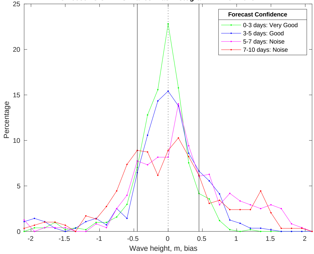
NDBC 46059 vs CMEMS Waves Bias Histogram: 24-Nov-2025
