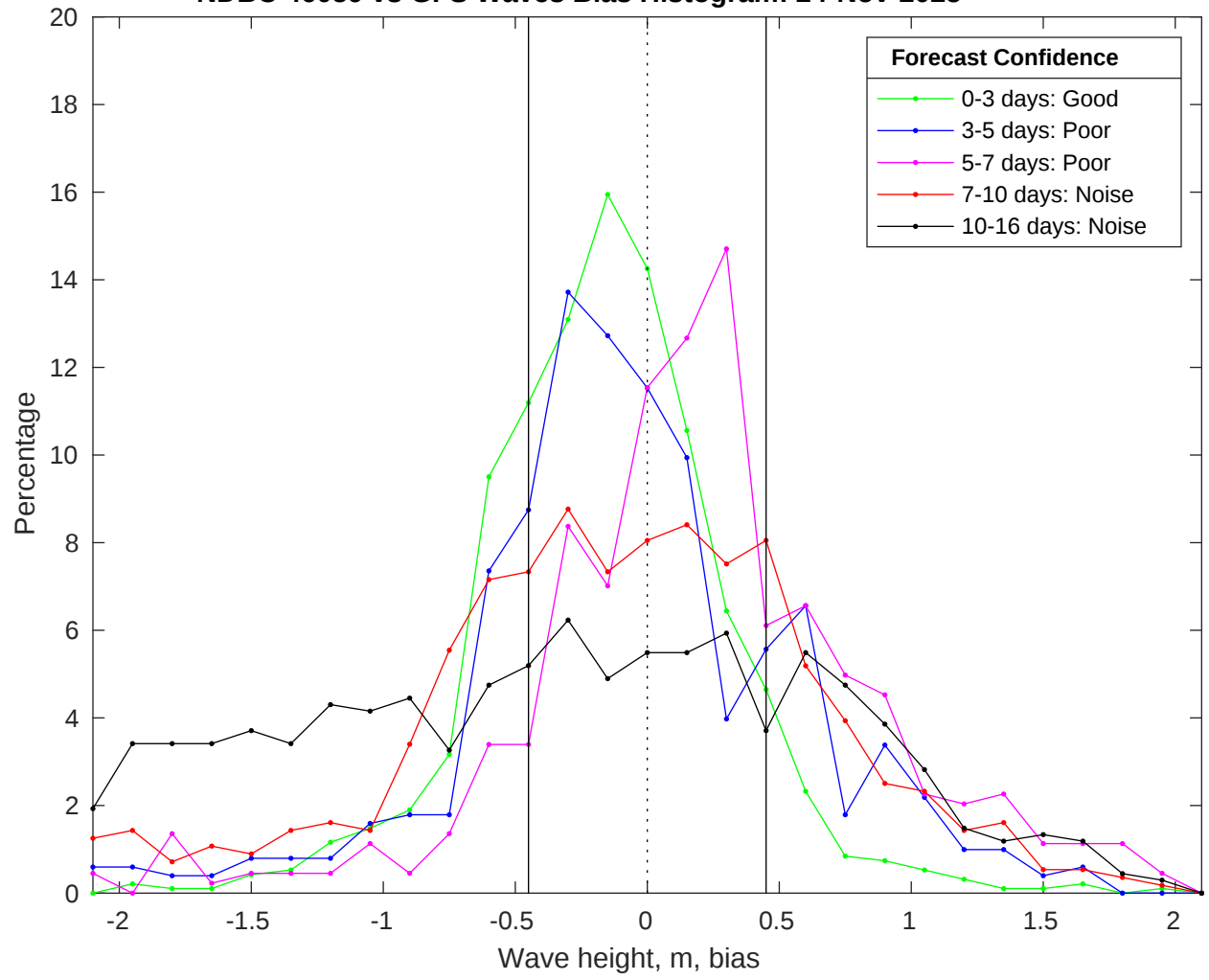
NDBC 46059 vs GFS Waves Bias Histogram: 24-Nov-2025
