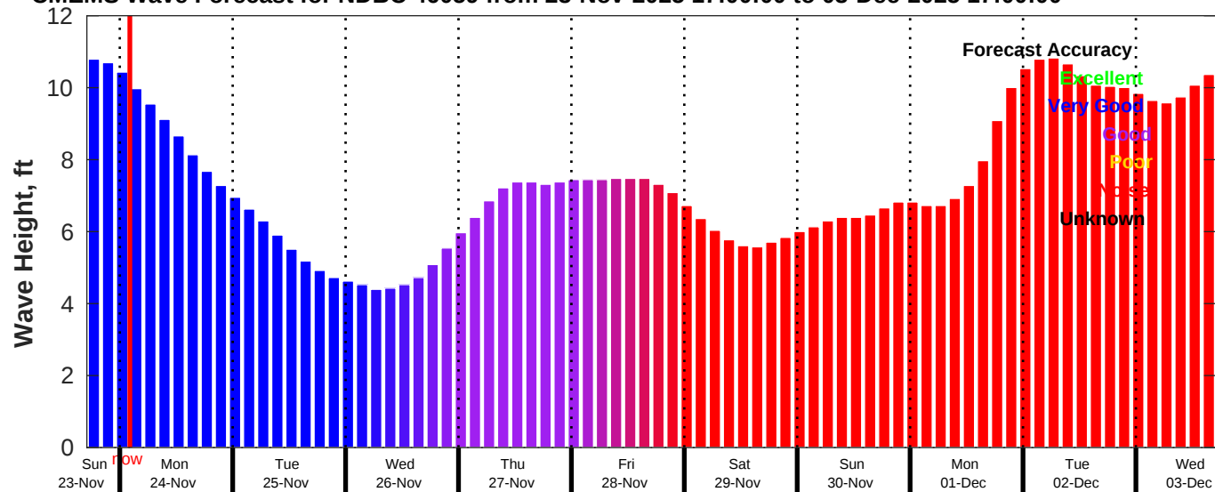
CMEMS Wave Forecast for NDBC 46059 from 23-Nov-2025 17:00:00 to 03-Dec-2025 17:00:00
