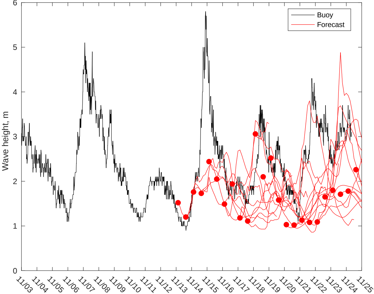
NDBC 46069 vs GFS Waves: 10 to 16 day forecast
