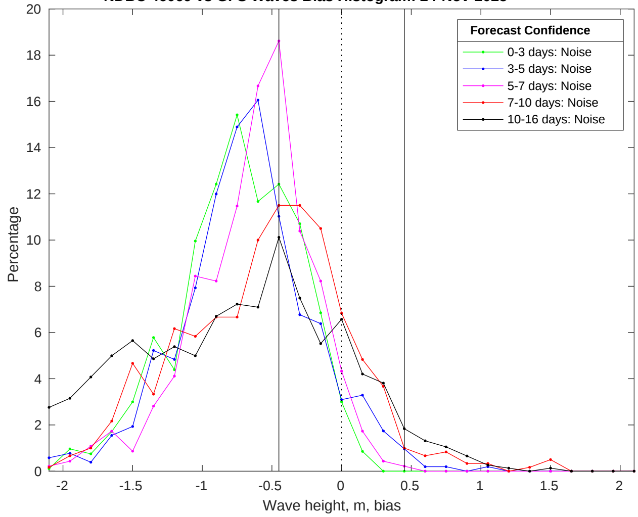
NDBC 46069 vs GFS Waves Bias Histogram: 24-Nov-2025
