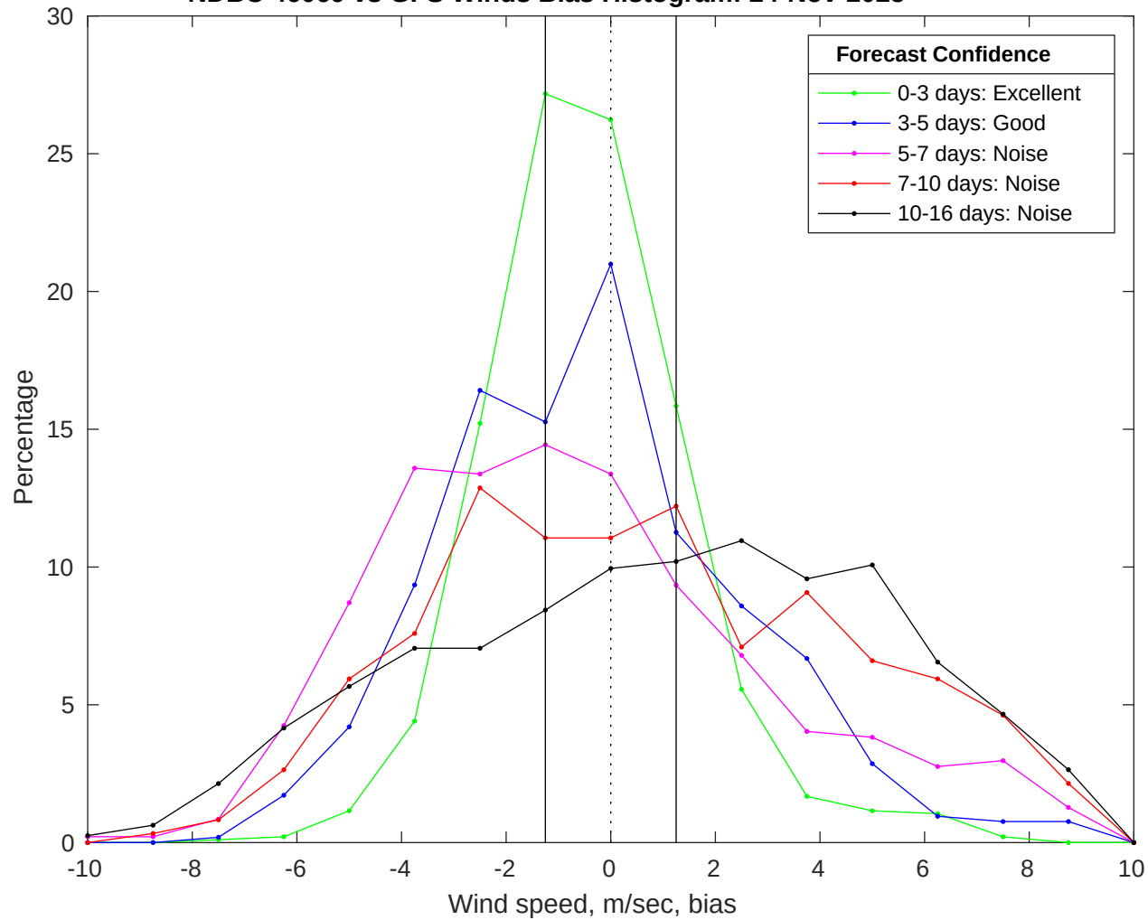
NDBC 46069 vs GFS Winds Bias Histogram: 24-Nov-2025
