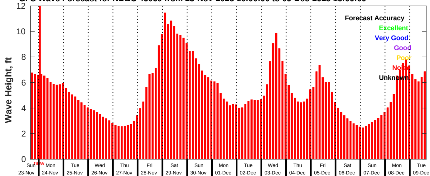
GFS Wave Forecast for NDBC 46069 from 23-Nov-2025 16:00:00 to 09-Dec-2025 16:00:00
