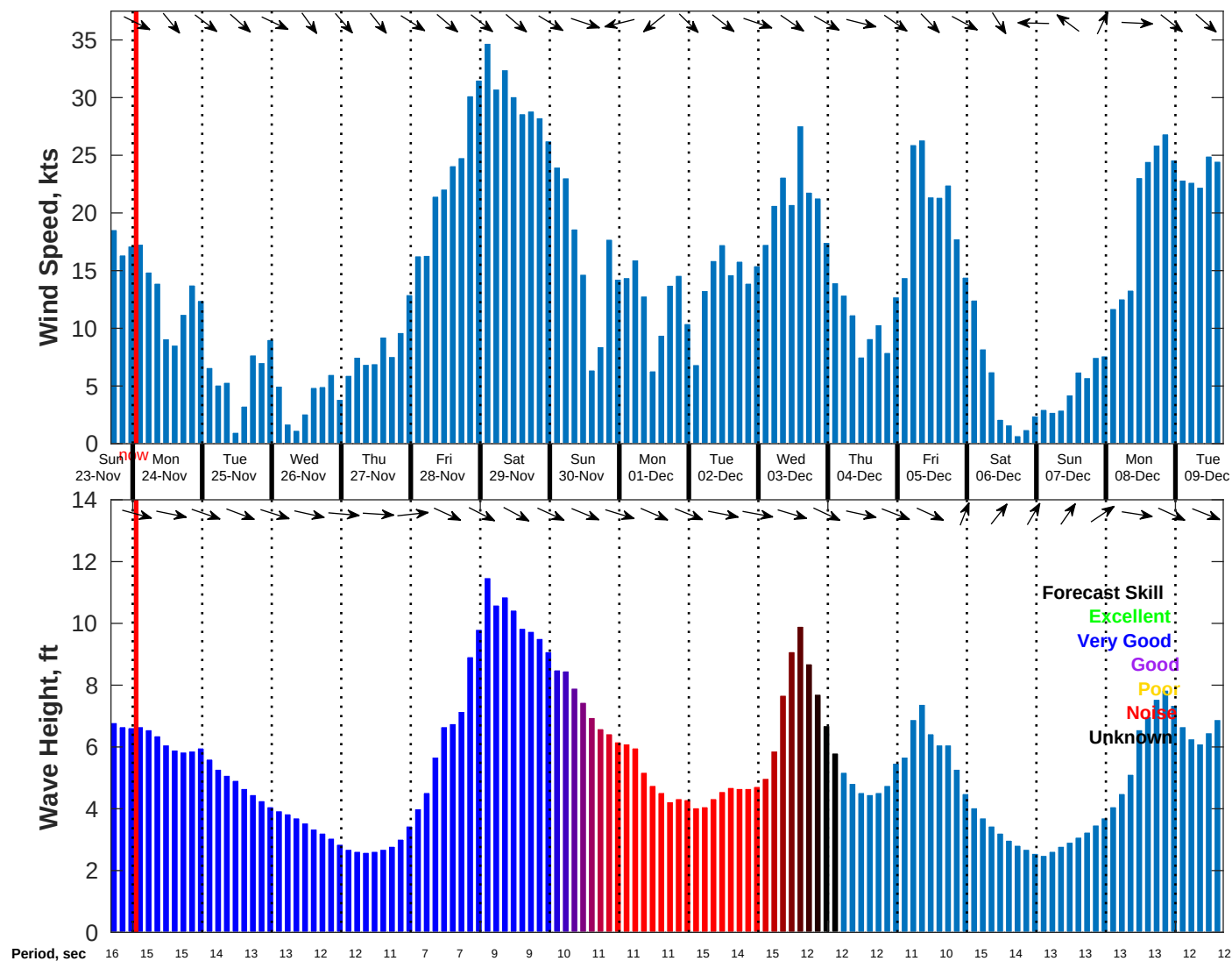
Wind & Wave Forecast for NDBC 46069 from 23-Nov-2025 16:00:00 to 09-Dec-2025 16:00:00
