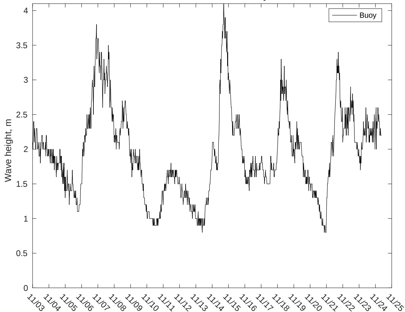
NDBC 46215 vs CMEMS Waves: 10 to 16 day forecast
