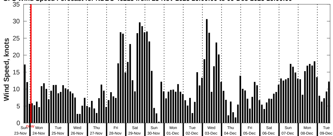
GFS Wind Speed Forecast for NDBC 46215 from 23-Nov-2025 16:00:00 to 09-Dec-2025 16:00:00
