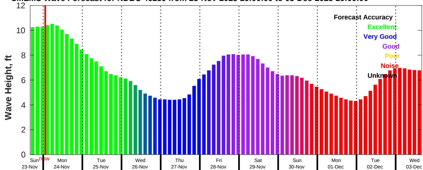
CMEMS Wave Forecast for NDBC 46259 from 23-Nov-2025 16:00:00 to 03-Dec-2025 16:00:00
