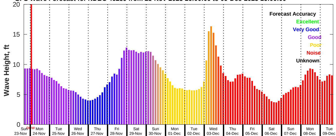
GFS Wave Forecast for NDBC 46259 from 23-Nov-2025 16:00:00 to 09-Dec-2025 16:00:00
