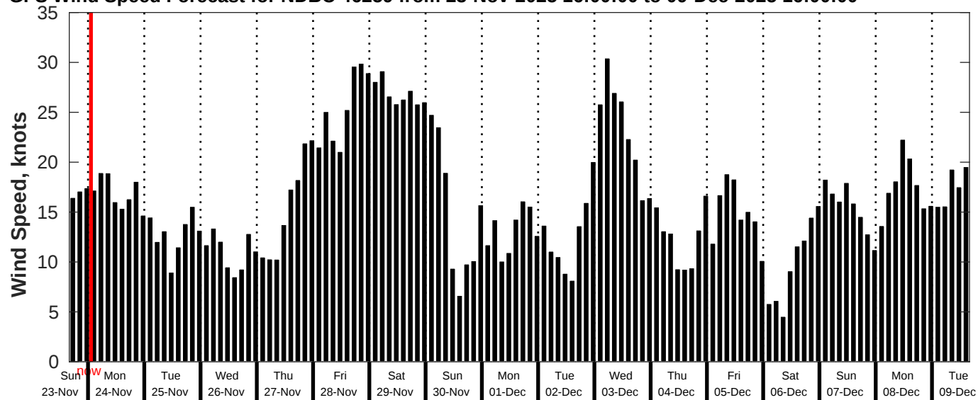
GFS Wind Speed Forecast for NDBC 46259 from 23-Nov-2025 16:00:00 to 09-Dec-2025 16:00:00
