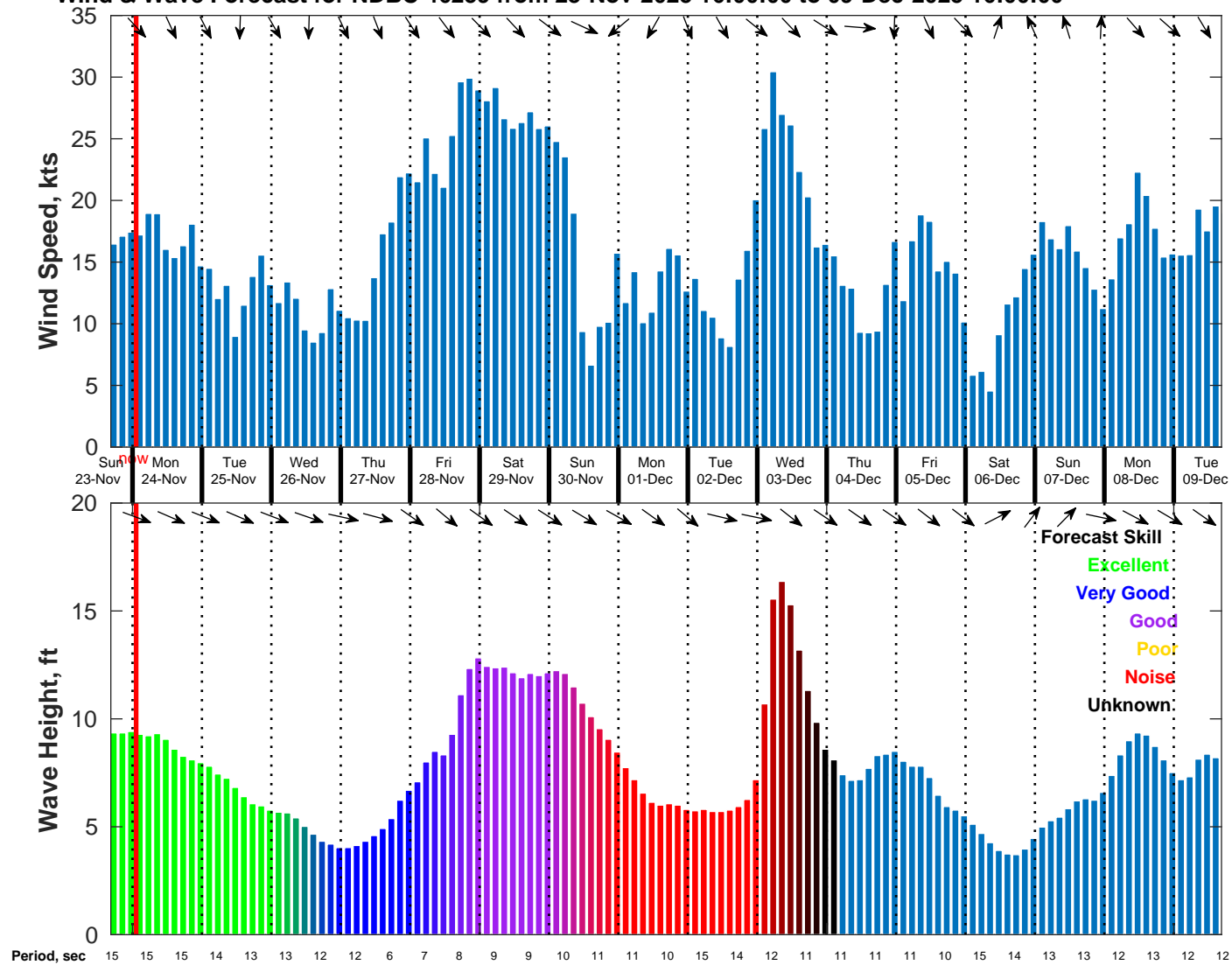
Wind & Wave Forecast for NDBC 46259 from 23-Nov-2025 16:00:00 to 09-Dec-2025 16:00:00
