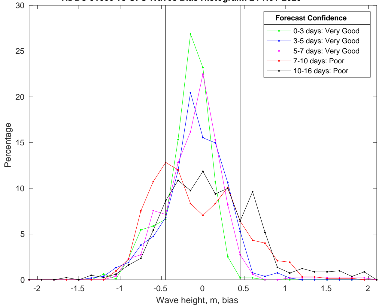
NDBC 51000 vs GFS Waves Bias Histogram: 24-Nov-2025
