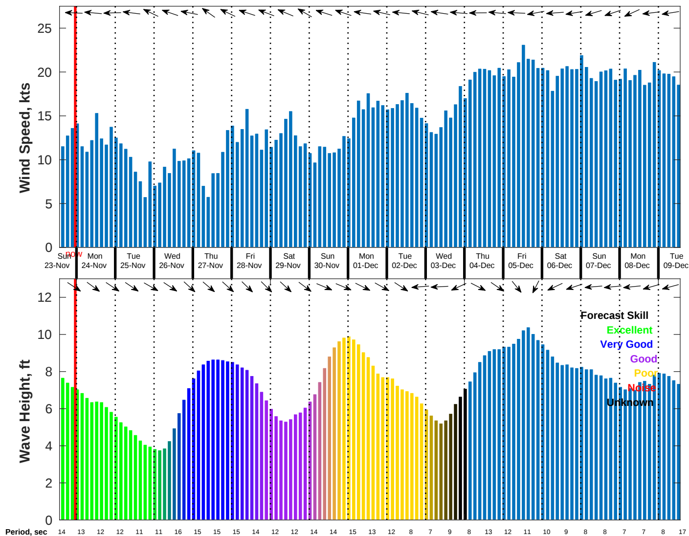
Wind & Wave Forecast for NDBC 51000 from 23-Nov-2025 14:00:00 to 09-Dec-2025 14:00:00
