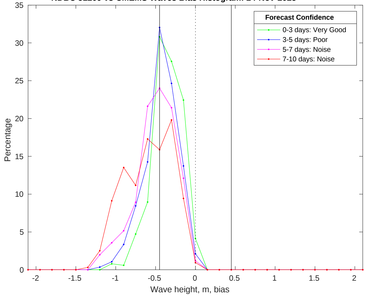
NDBC 51209 vs CMEMS Waves Bias Histogram: 24-Nov-2025
