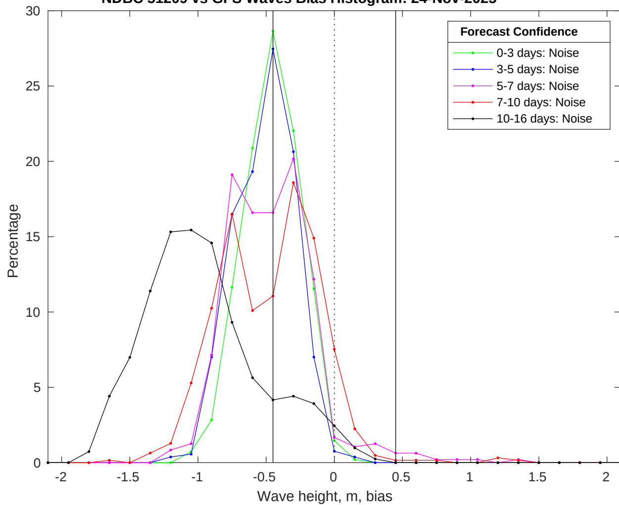
NDBC 51209 vs GFS Waves Bias Histogram: 24-Nov-2025
