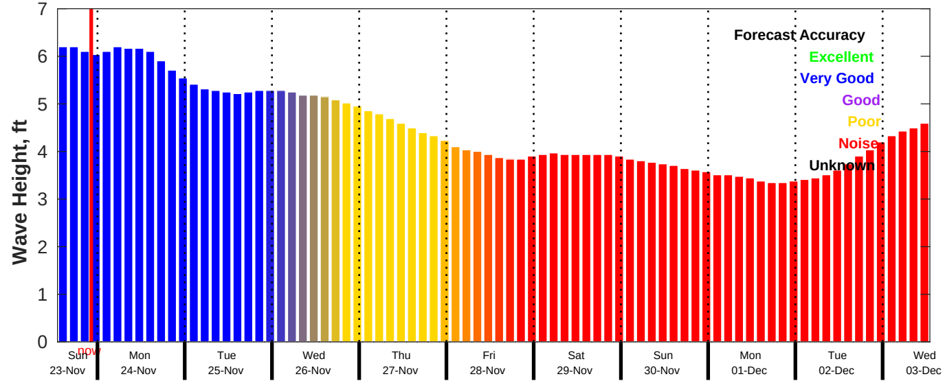
CMEMS Wave Forecast for NDBC 51209 from 23-Nov-2025 13:00:00 to 03-Dec-2025 13:00:00
