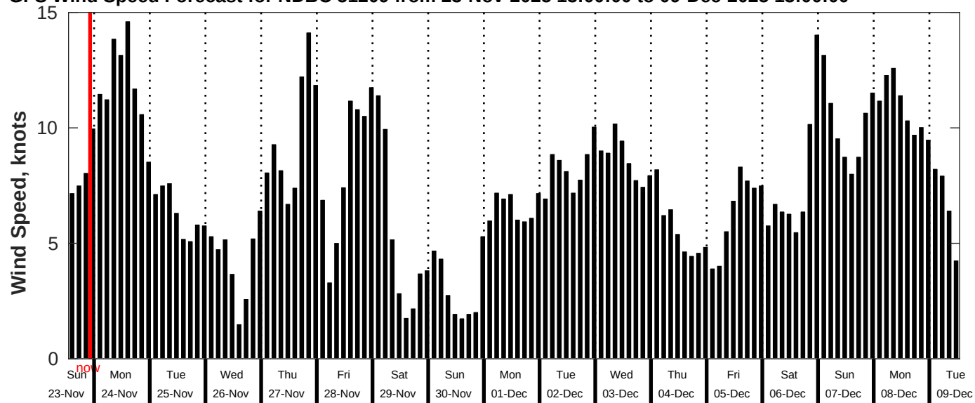
GFS Wind Speed Forecast for NDBC 51209 from 23-Nov-2025 13:00:00 to 09-Dec-2025 13:00:00
