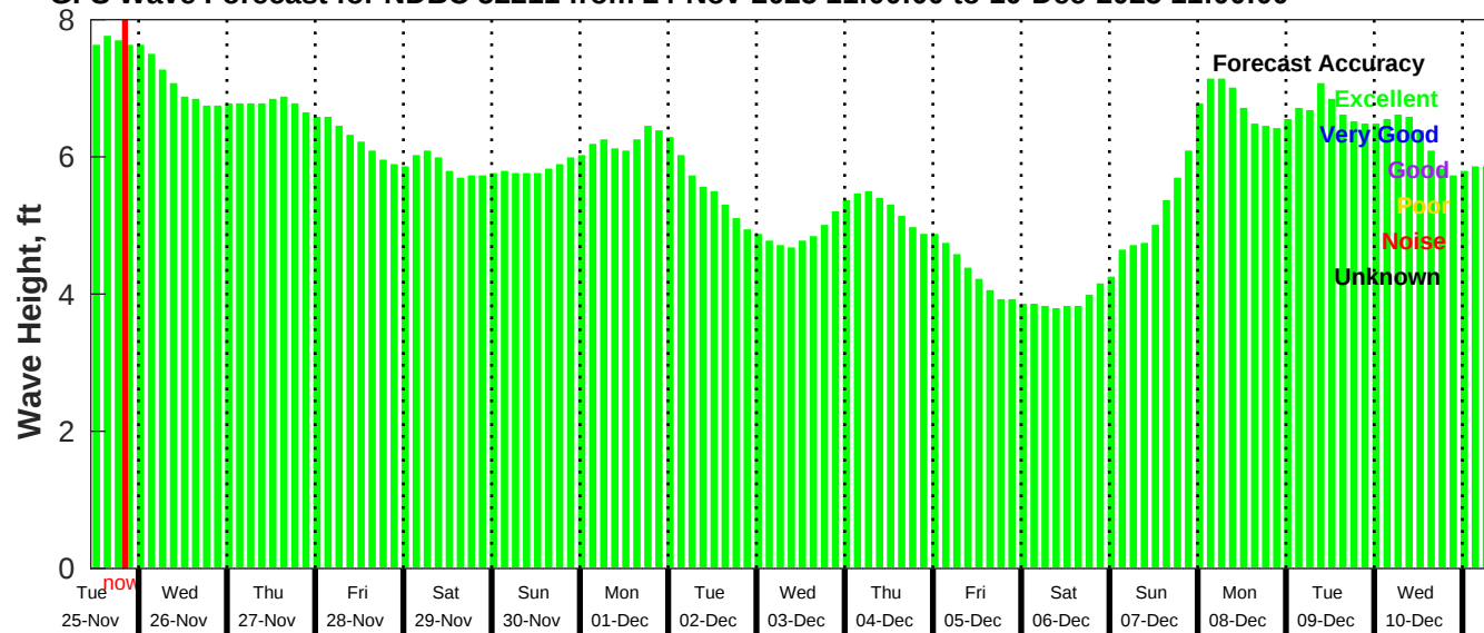
GFS Wave Forecast for NDBC 52211 from 24-Nov-2025 11:00:00 to 10-Dec-2025 11:00:00
