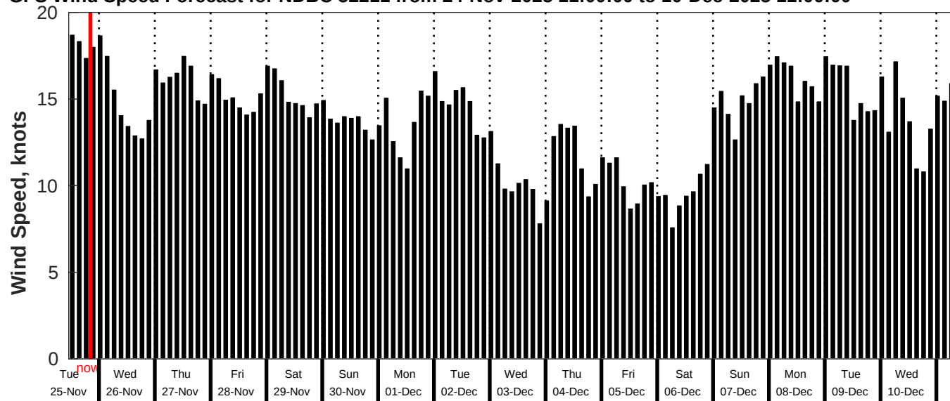
GFS Wind Speed Forecast for NDBC 52211 from 24-Nov-2025 11:00:00 to 10-Dec-2025 11:00:00
