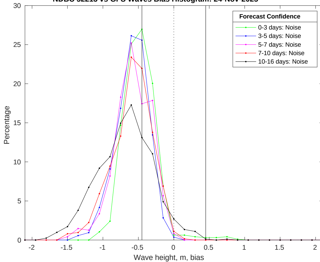
NDBC 52213 vs GFS Waves Bias Histogram: 24-Nov-2025
