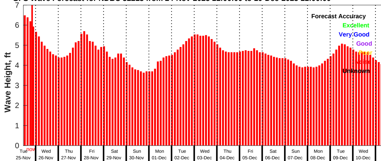
GFS Wave Forecast for NDBC 52213 from 24-Nov-2025 11:00:00 to 10-Dec-2025 11:00:00
