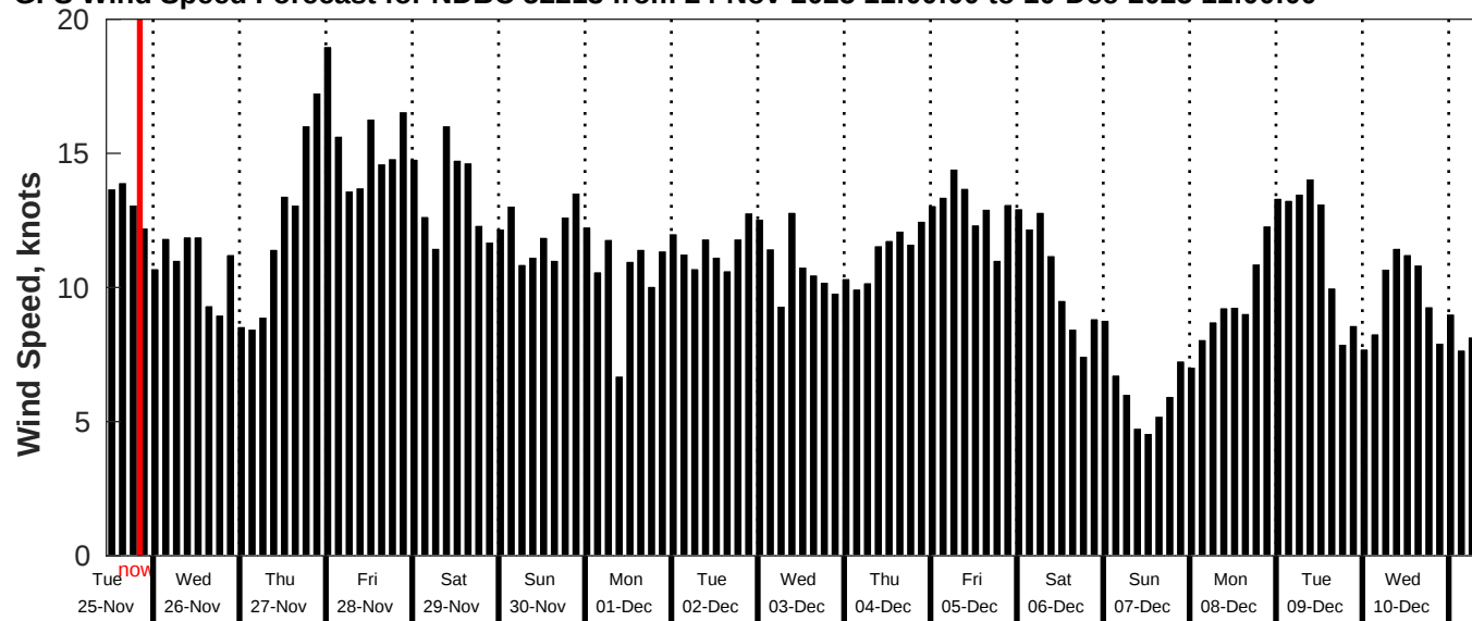
GFS Wind Speed Forecast for NDBC 52213 from 24-Nov-2025 11:00:00 to 10-Dec-2025 11:00:00
