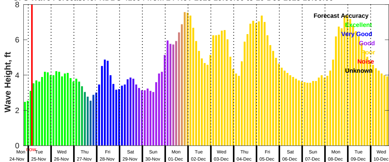
GFS Wave Forecast for NDBC 41004 from 24-Nov-2025 19:00:00 to 10-Dec-2025 19:00:00
