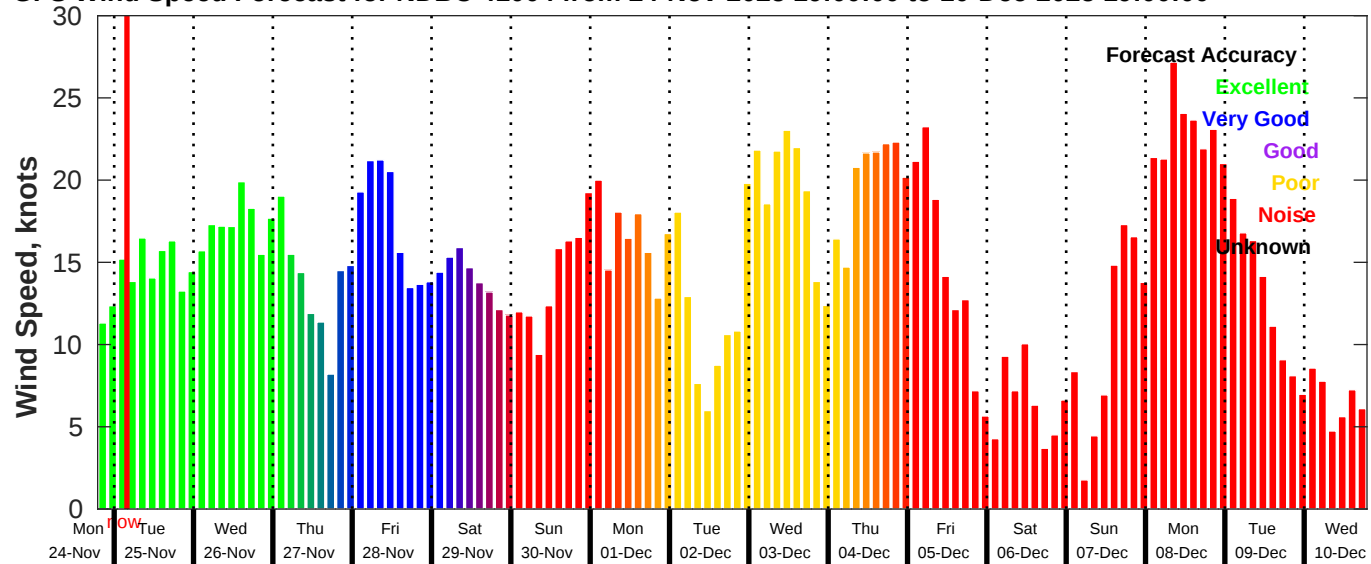
GFS Wind Speed Forecast for NDBC 41004 from 24-Nov-2025 19:00:00 to 10-Dec-2025 19:00:00
