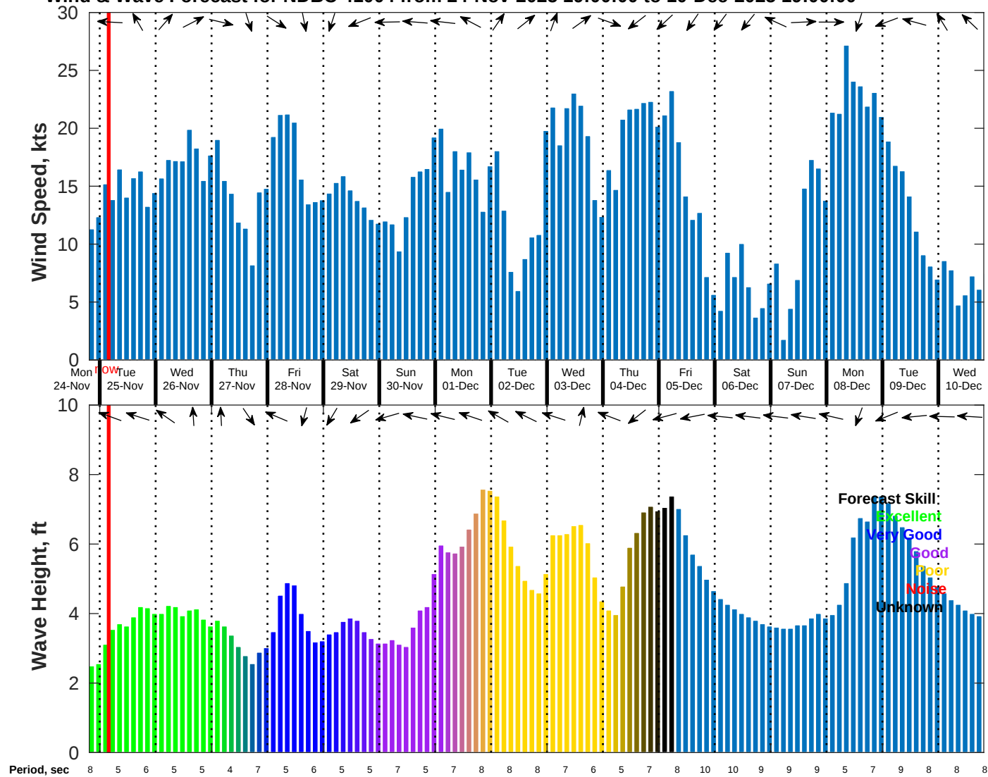
Wind & Wave Forecast for NDBC 41004 from 24-Nov-2025 19:00:00 to 10-Dec-2025 19:00:00
