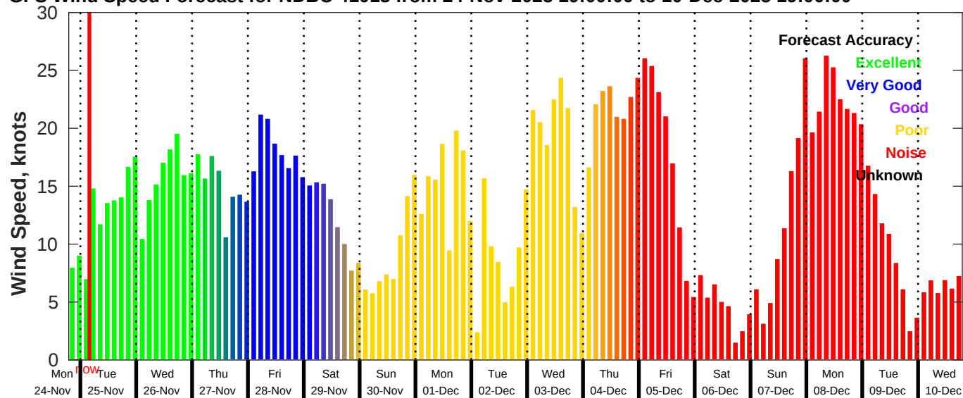
GFS Wind Speed Forecast for NDBC 41013 from 24-Nov-2025 19:00:00 to 10-Dec-2025 19:00:00
