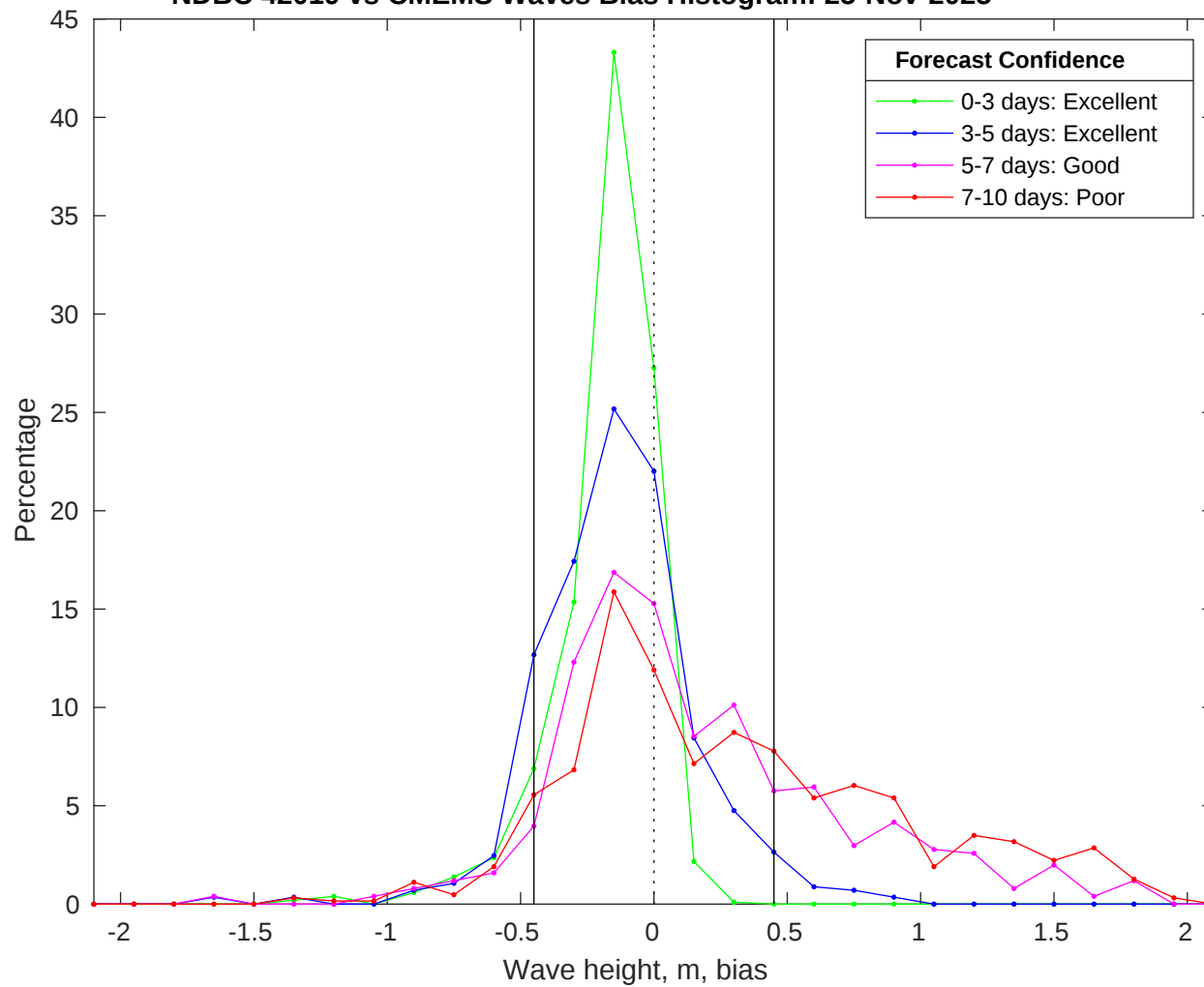
NDBC 42019 vs CMEMS Waves Bias Histogram: 25-Nov-2025
