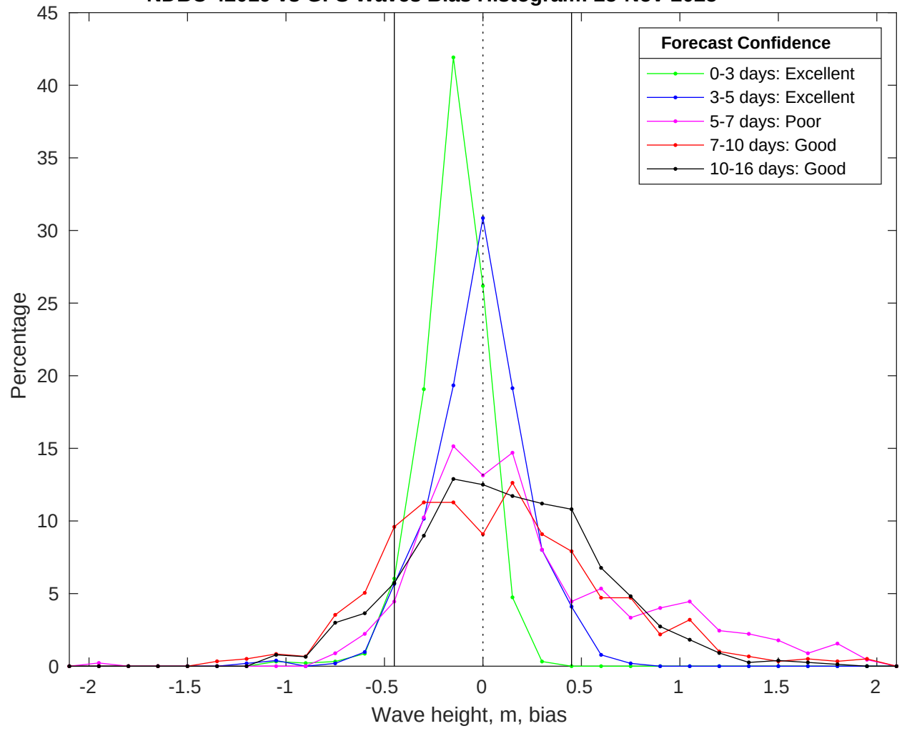
NDBC 42019 vs GFS Waves Bias Histogram: 25-Nov-2025
