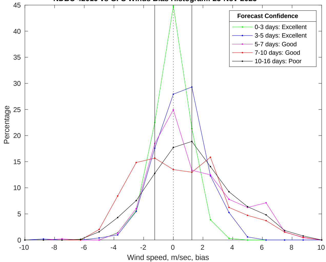
NDBC 42019 vs GFS Winds Bias Histogram: 25-Nov-2025
