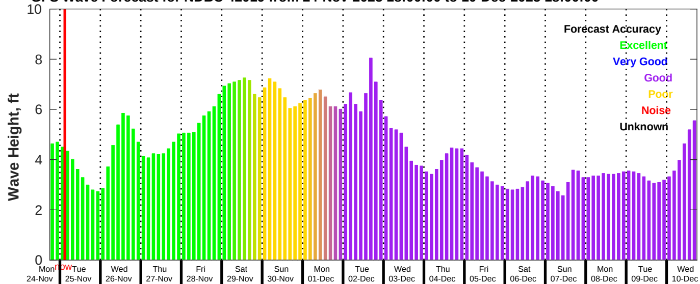
GFS Wave Forecast for NDBC 42019 from 24-Nov-2025 18:00:00 to 10-Dec-2025 18:00:00
